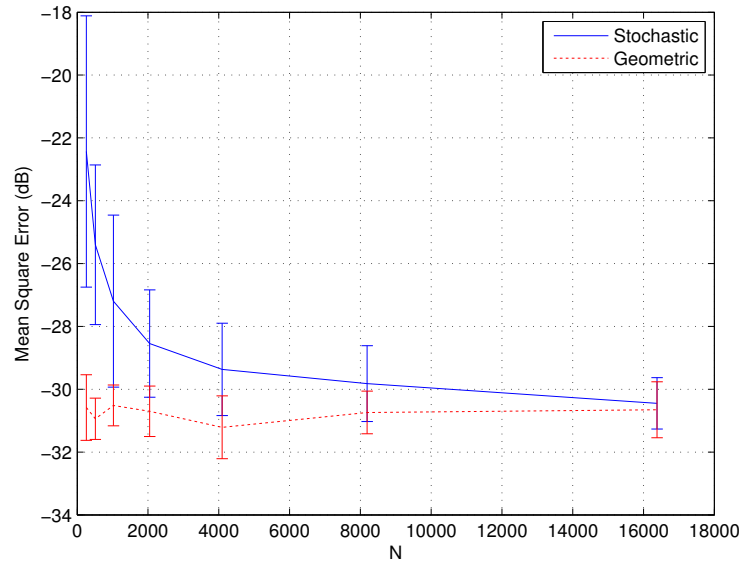
Figure 1: Mean square error in dB between the measured and theoretical spatial coherence for N = 2^n , with n = 8, 9, \dots, 14 .
